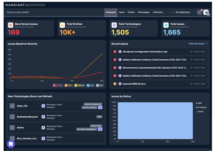
FIGURE 2. Manage changes in the attack surface over time, empowered by the world's foremost threat intelligence and expertise.
