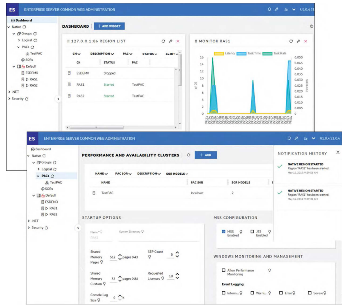
Fig 2. Rocket Enterprise Server Web Administration for managing Enterprise Server resources.
