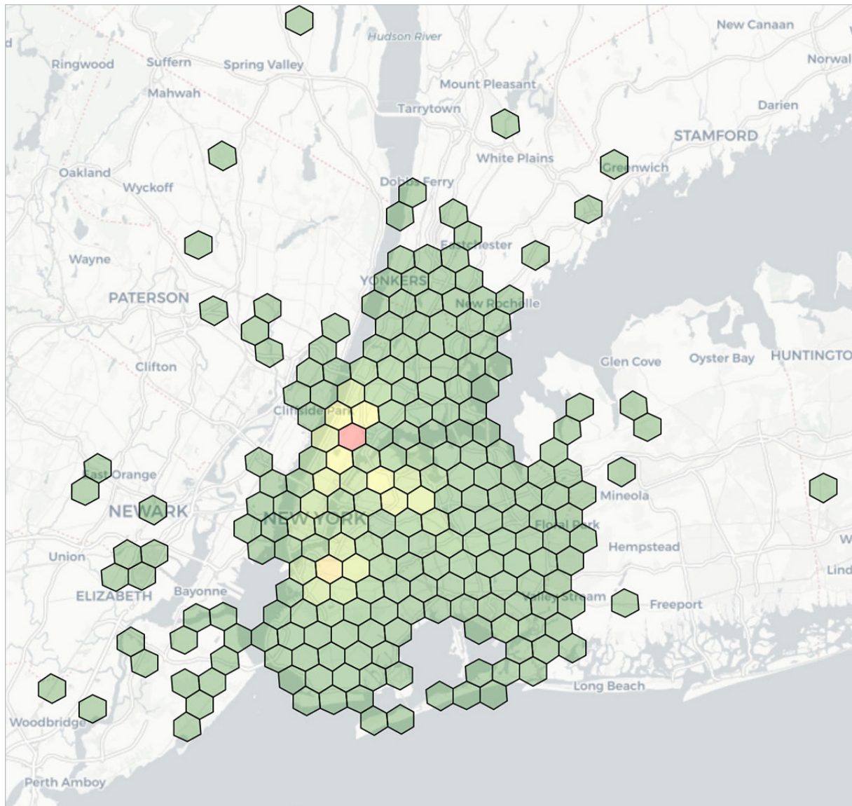
Example: Geospatial visualization of taxi dropoff locations, with latitude and longitude binned at a resolution of 7 (1.22km edge length) and colored by aggregated counts within each bin
