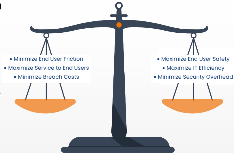
Authentication Tradeoffs
