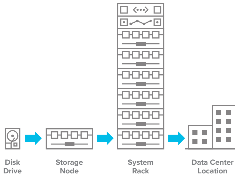
Figure 5 - Storage Hierarchy
