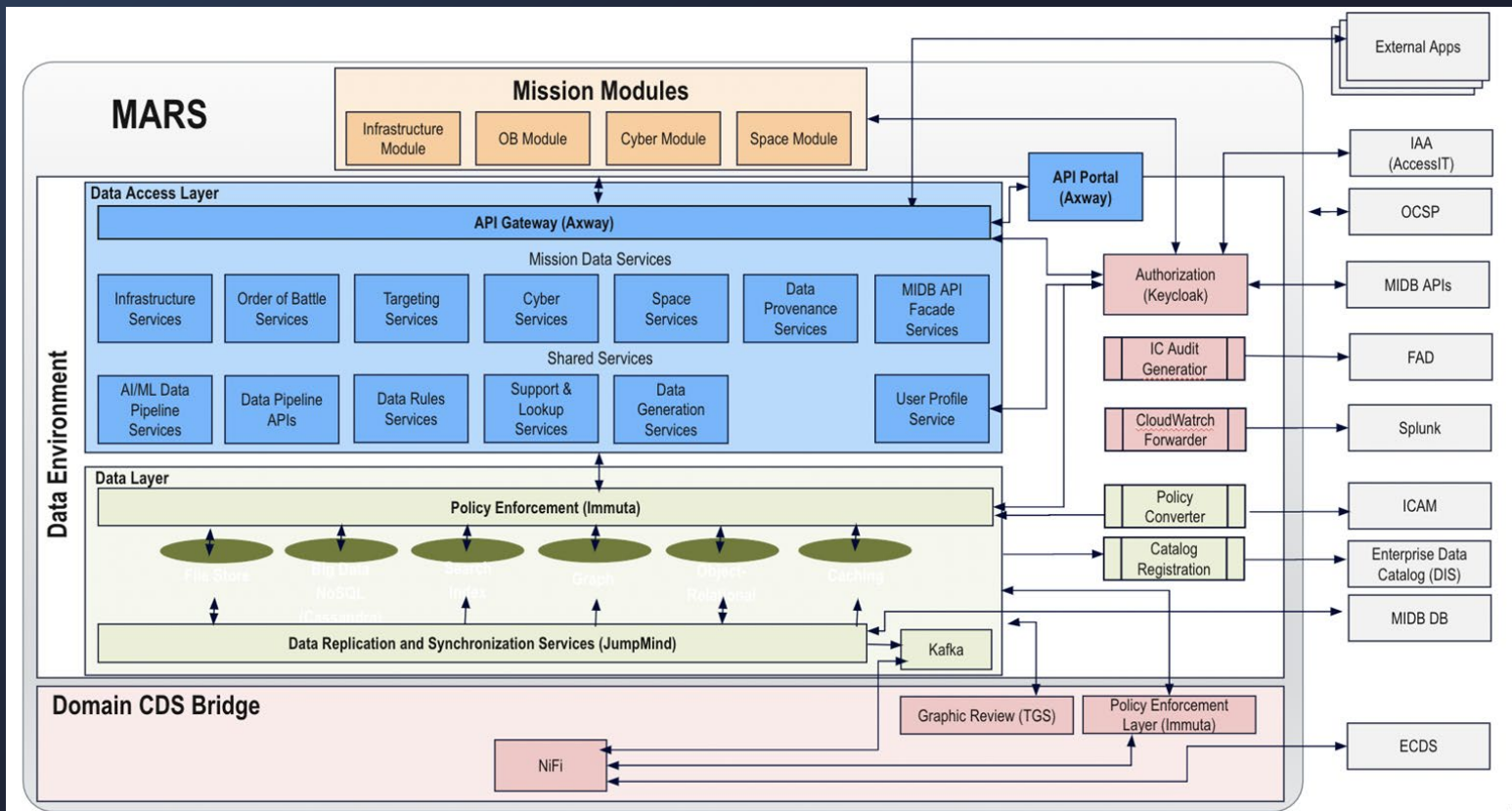
Diagram 2: MARS Target Architecture with Zero-trust elements
