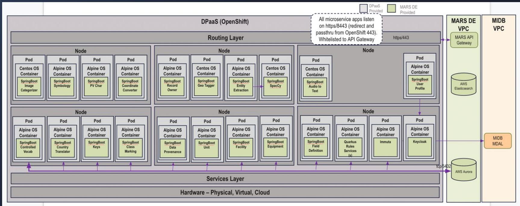
Diagram 1: MARS DPaaS Integration Architecture
