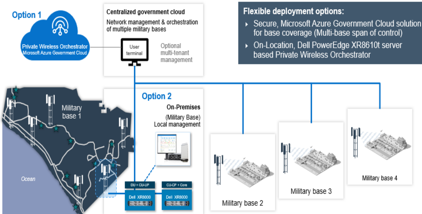
Figure 3: Simplified management of multiple military bases enabled by Dell Private Wireless Orchestrator's flexible deployment options
